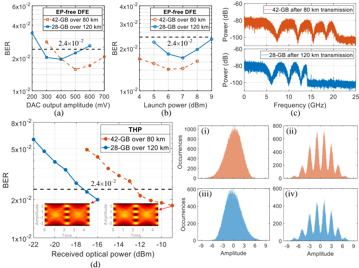
Fig. 3. (a) BER versus DAC output amplitude for 42-Gbaud and 28-Gbaud PAM4 signals. (b) BER versus launch for 42-Gbaud and 28-Gbaud PAM4 signals. (c) The detected spectra of 42-Gbaud and 28-Gbaud PAM4 signals. (d) BER versus ROP for 42-Gbaud and 28-Gbaud PAM4 signals. Inset (i-ii) The histograms of 42-Gbaud PAM4 signals before and after FFE at -9 -dB ROP, respectively. Inset (iii-iv) The histograms of 28-Gbaud PAM4 signals before and after FFE at -16 -dB ROP, respectively.
