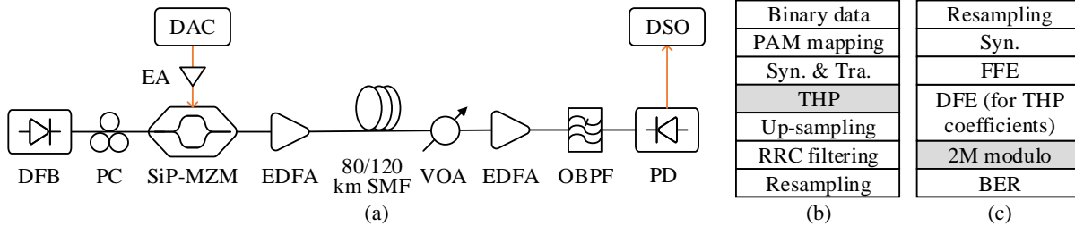
Fig. 2 (a) Experimental setup of the SiP-MZM-based IM/DD system. (b) Tx DSP flow charts. (c) Rx DSP flow charts. The THP and 2M modulo in the grey blocks are performed only if the THP is employed.
