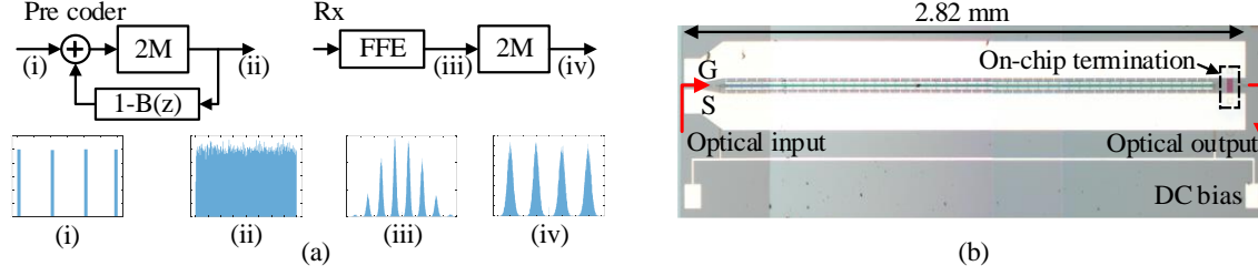
Fig. 1 (a) The schematic diagram of the THP technique. Inset (i-iv) The histograms of input signal, transmitted signal, equalized signal, and recovered signal, respectively. (b) The micrograph of the SiP-MZM.
